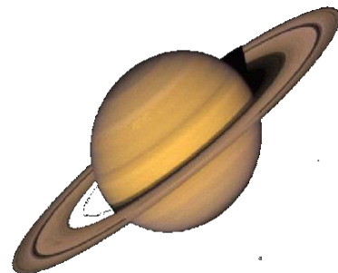
Saturn
