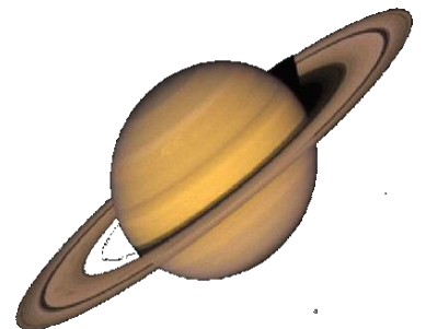
Saturn
