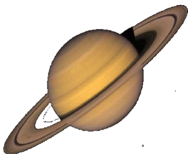
Saturn
