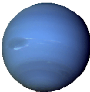
Neptune
