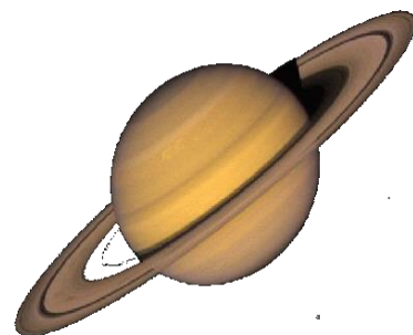
Saturn
