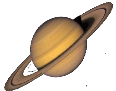
Saturn
