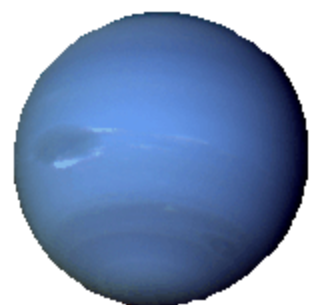
Neptune
